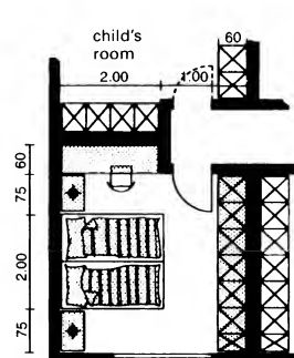
⑫ Bedroom with adjacent child's room
